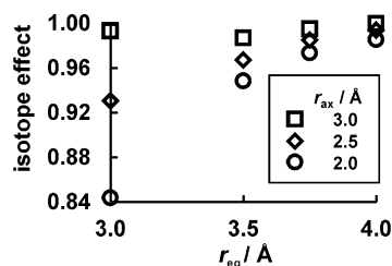
Figure 2. 2° D 3 EIEs (298 K) for the transfer of axial [ \text{H}_2\text{O}\cdots\text{CH}_3^+\cdots\text{OH}_2 ] structures from the vacuum into the center of the equatorial ring of the constrained cage.
