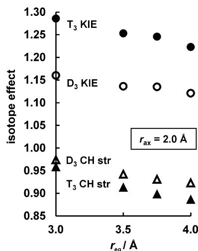
Figure 3. Influence of equatorial CH···O interactions ( r_{\text{eq}} ) on 2° T 3 and D 3 KIEs (298 K) for methyl transfer within a superheavy constrained cage with r_{\text{ax}}=2 Å, along with contributions of CH stretching modes of the complexes.
