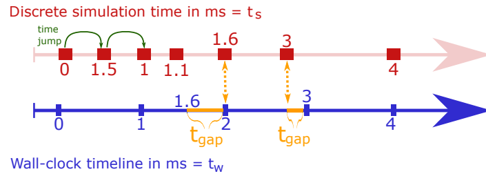
Figure 2. Visualisation of t_{gap} between the t_{s1} = 1.6\text{ ms} and W2S(t_{w1}) = 2\text{ ms} .
