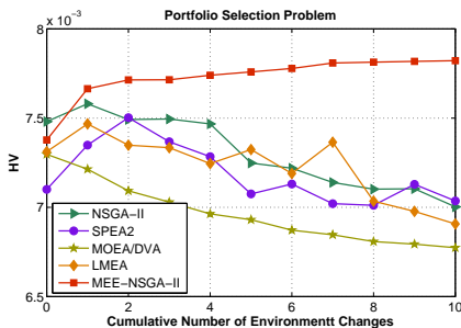
Figure 4: Average of HV over 20 runs versus time on the portfolio selection problem
