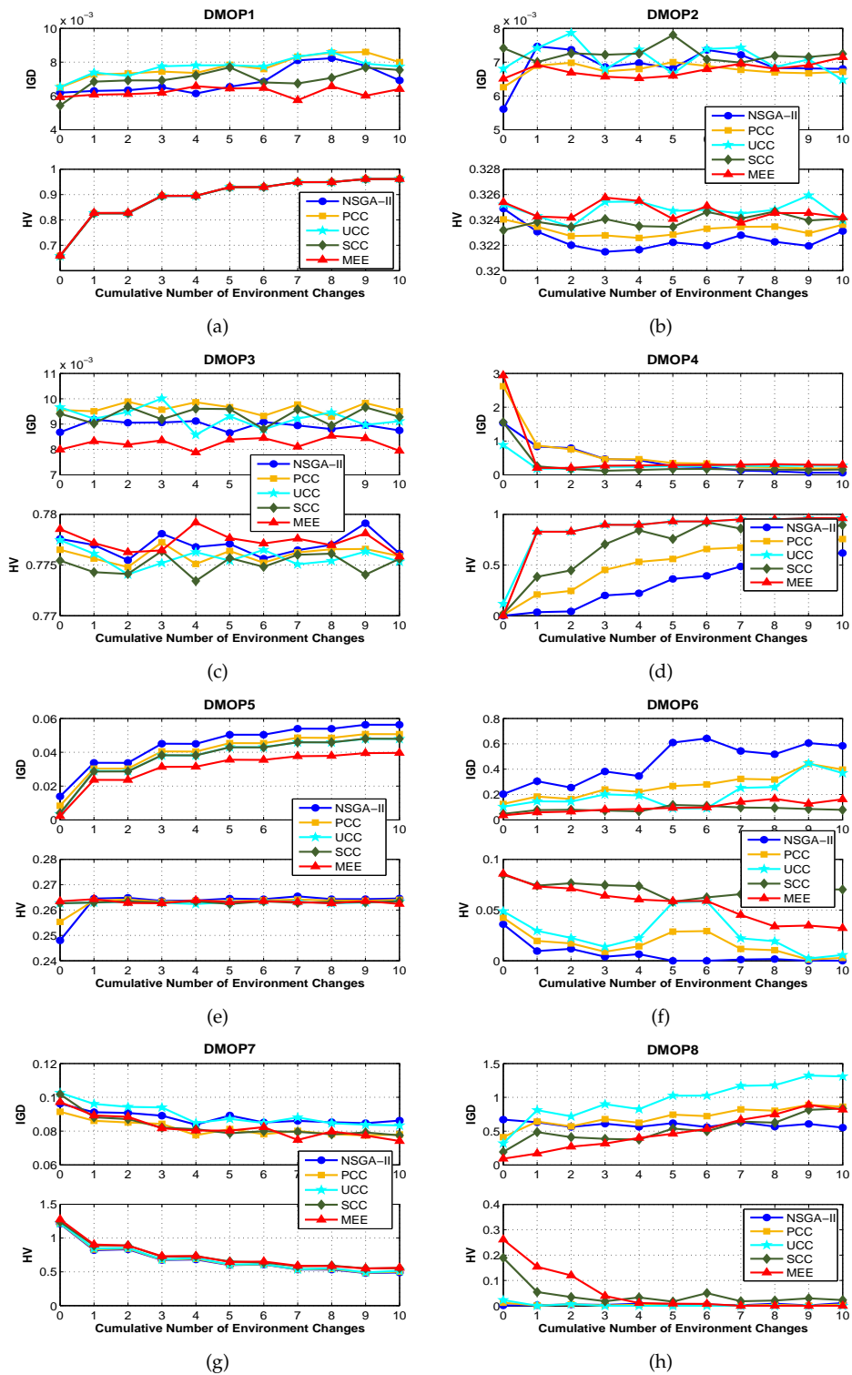
Figure 3: Averages of IGD and HV over 30 runs versus time on DMOP1-DMOP8
