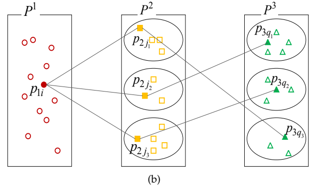
Figure 2: Process of evaluating an individual in a sub-population
