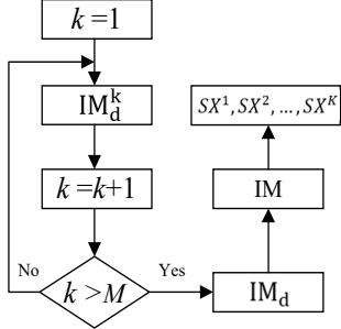
Figure 1: Flow chart of forming initial groups of decision variables for an MOP
