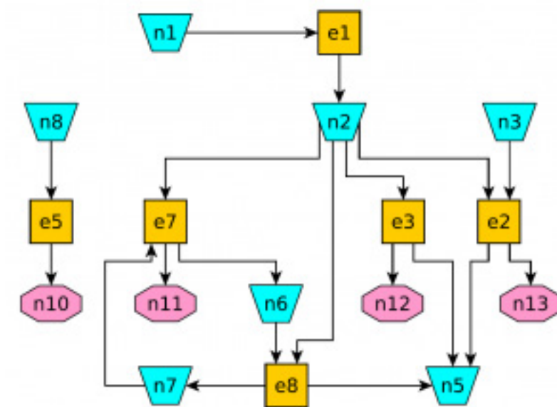
Figure 5 Example of a transformation graph
