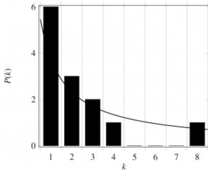
Figure 6 Degree distribution in the example presented in Figure 1.
