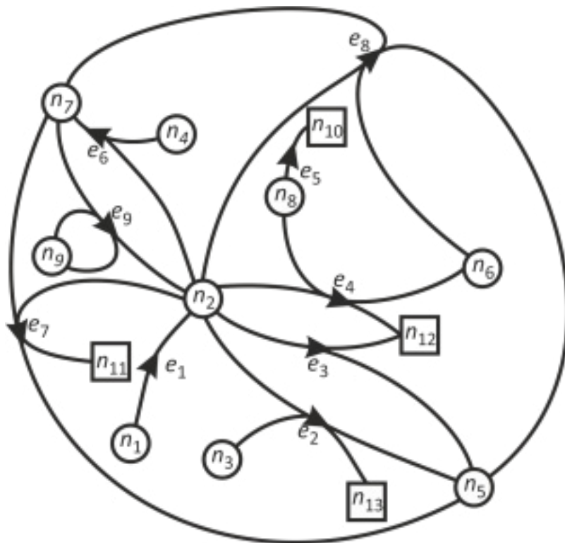
Figure 1 A directed hypergraph representing a simplified utility-service provision problem.
