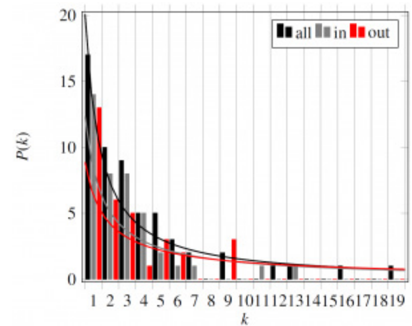
Figure 7 Degree distribution in the mastergraph.
