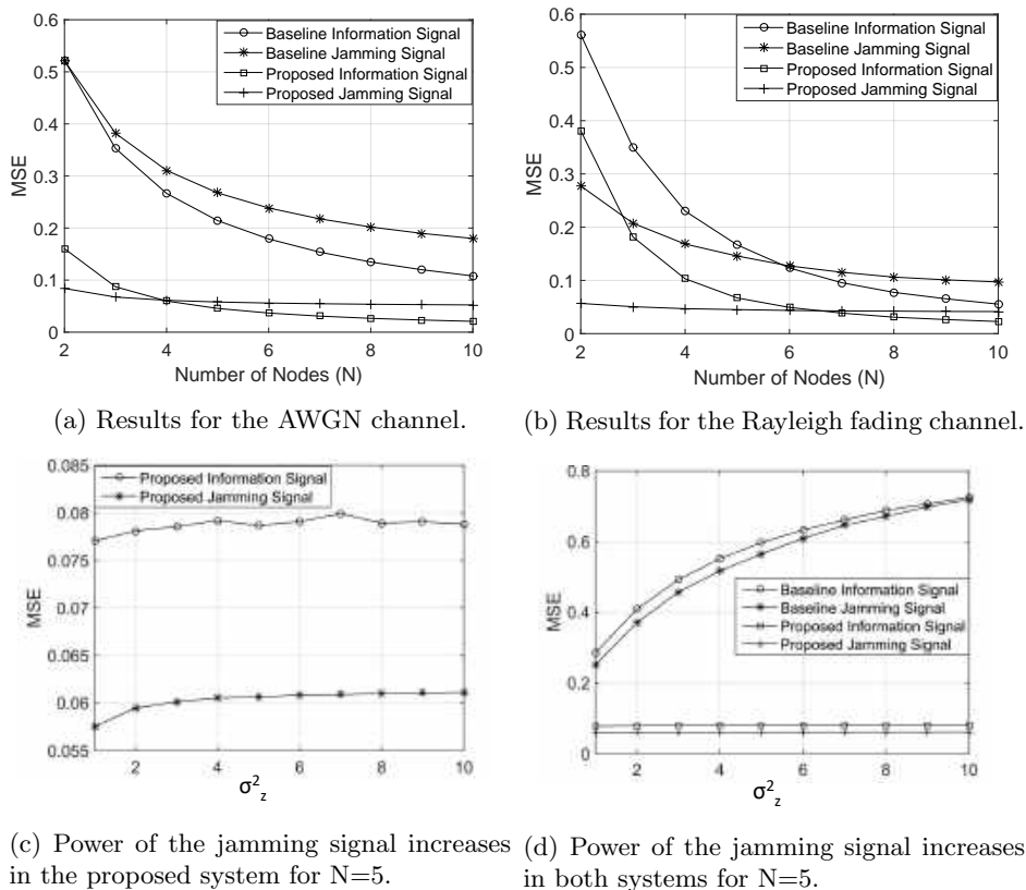
Fig. 2: Information and Jamming Signal Estimation
