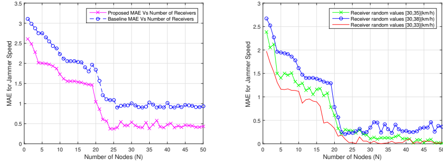
(a) Comparing the proposed with the baseline method. (b) Different ranges for the speed of the receivers.
